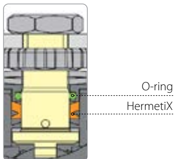
Double stem sealing
