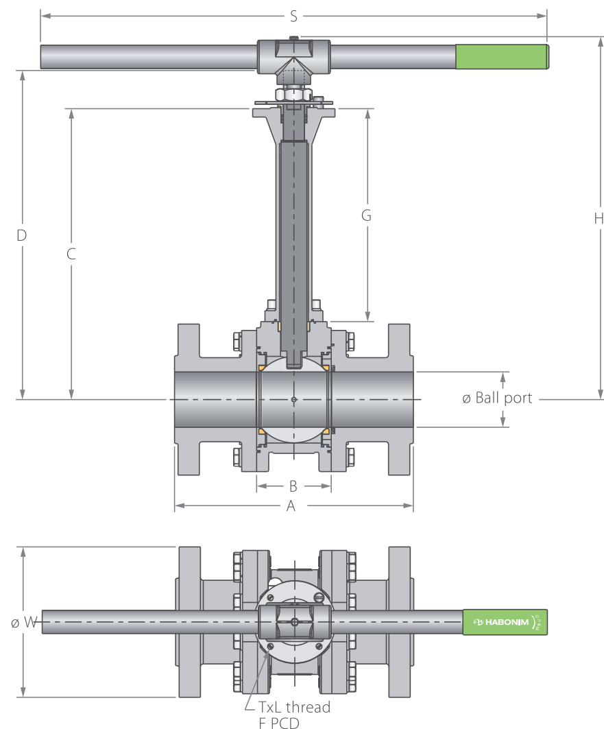
Valve dimensions
