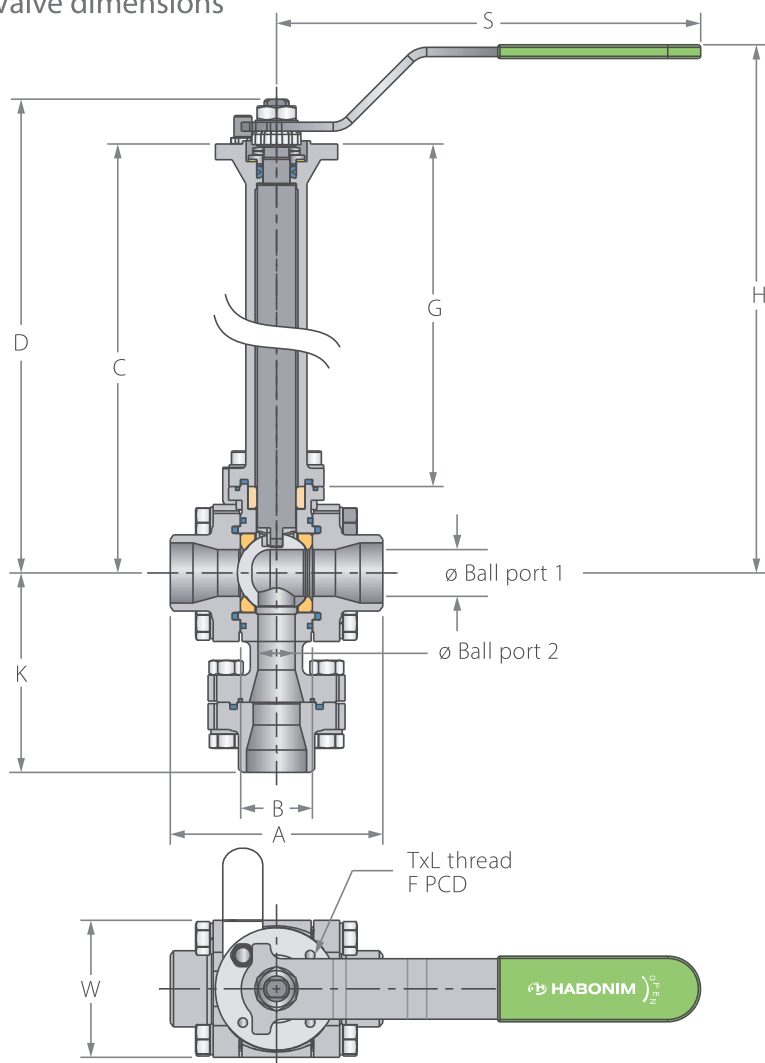
Valve dimensions
